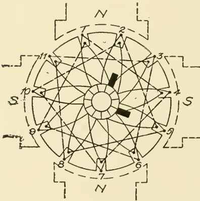
Fig. 37. Diagram of Armature Winding
